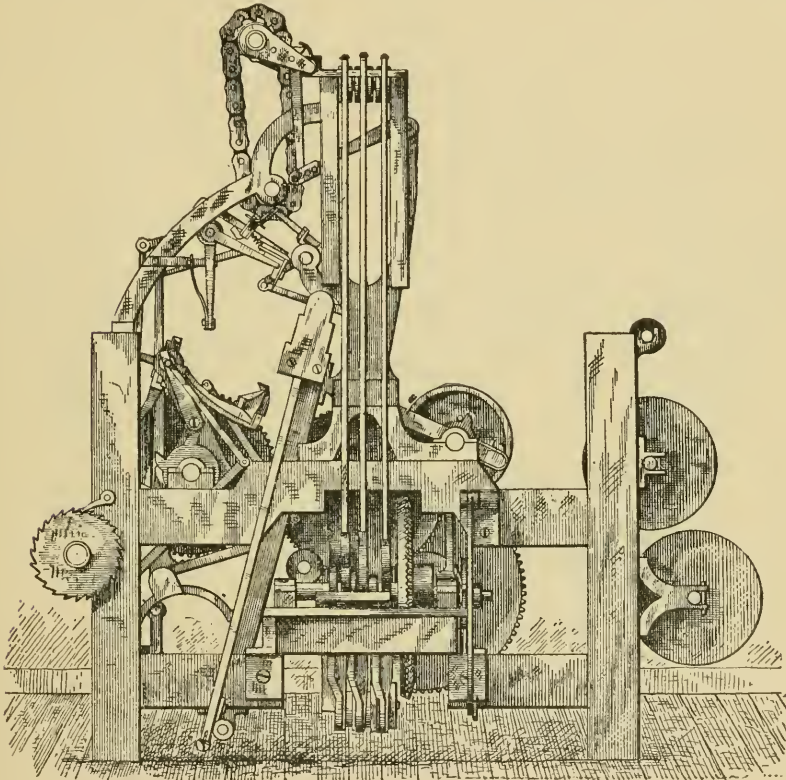
SMITH AND SKINNER LOOM FOR MOQUETTE CARPETS.
